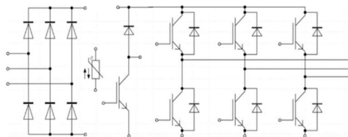
Equivalent Circuit Schematic
