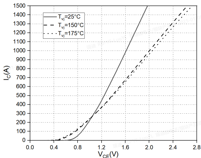
Output characteristic IGBT, Inverter (typical), Inclusive R_{CC'+EE'}
